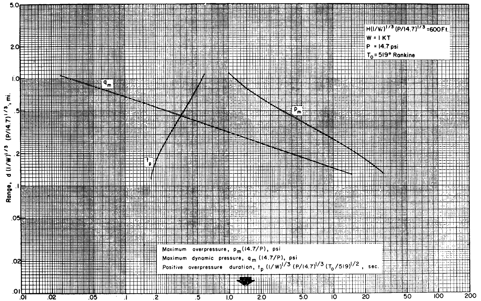
Fig. 2.7—Scaled blast parameters for a scaled height of burst of 600 ft as a function of scaled range. These are plots of Eqs. 2.48, 2.50, and 2.52 given in Table 2.7.
